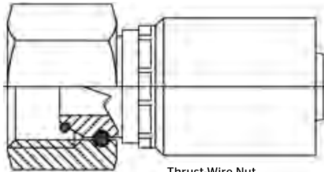
Thrust-Wire Nut
