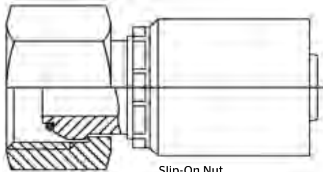
Slip-On Nut
