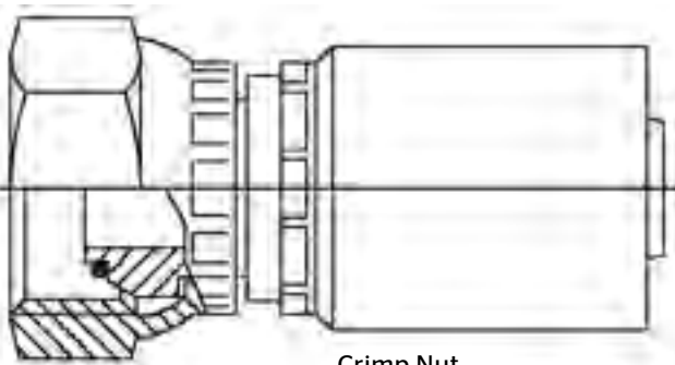
Crimp Nut
